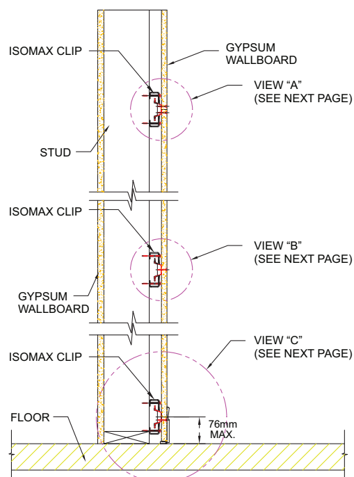
WALL/FLOOR SECTION
