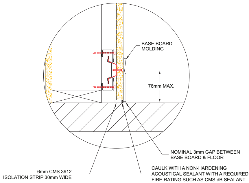
ENLARGED VIEW "C"
